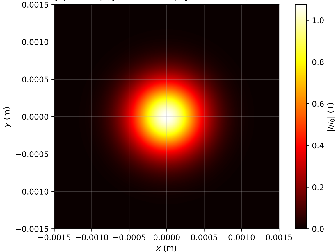
Intensity profile I(x, y, z = 0.318m)/I_0 , Pin=1.0Pcr, artificial time
